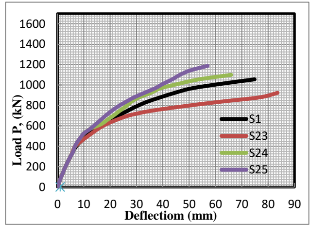
(h) Effect of Compression steel ratio/ \mu_{max} ( \mu'/\mu_{max} )
