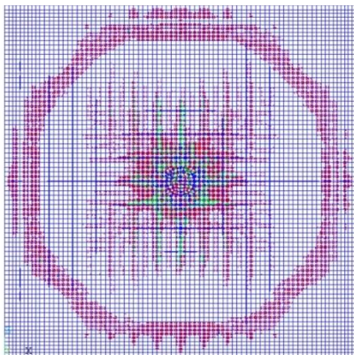
(a) Predicted cracks pattern.
