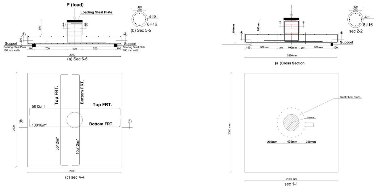
Fig.6 Geometry and reinforcement details of the parametric studied slabs.
