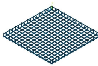
(b) Reinforcing bar elements (Link 180)
