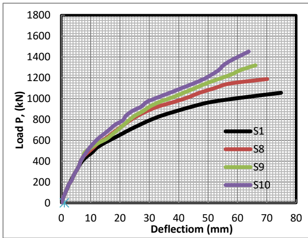
(c) Effect of slab thickness ( t_s )
