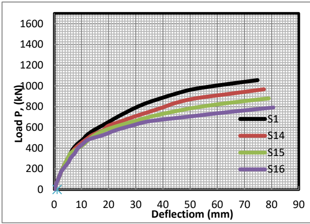
(e) Effect of shear studs spacing / t_s ratio ( S_b/t_s )
