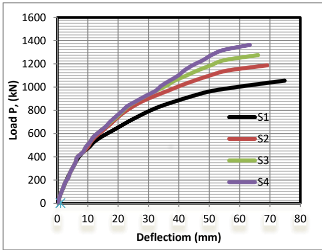
(a) Effect of concrete compressive strength f_{cu}
