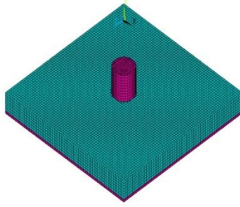
(a) Concrete elements (Solid 65)
