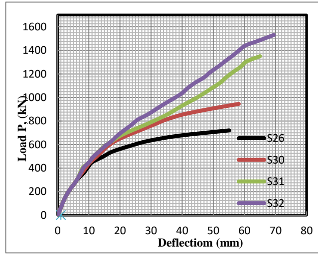
(j) Effect of drop panel diameter/ t_s ratio ( D_d/t_s )
