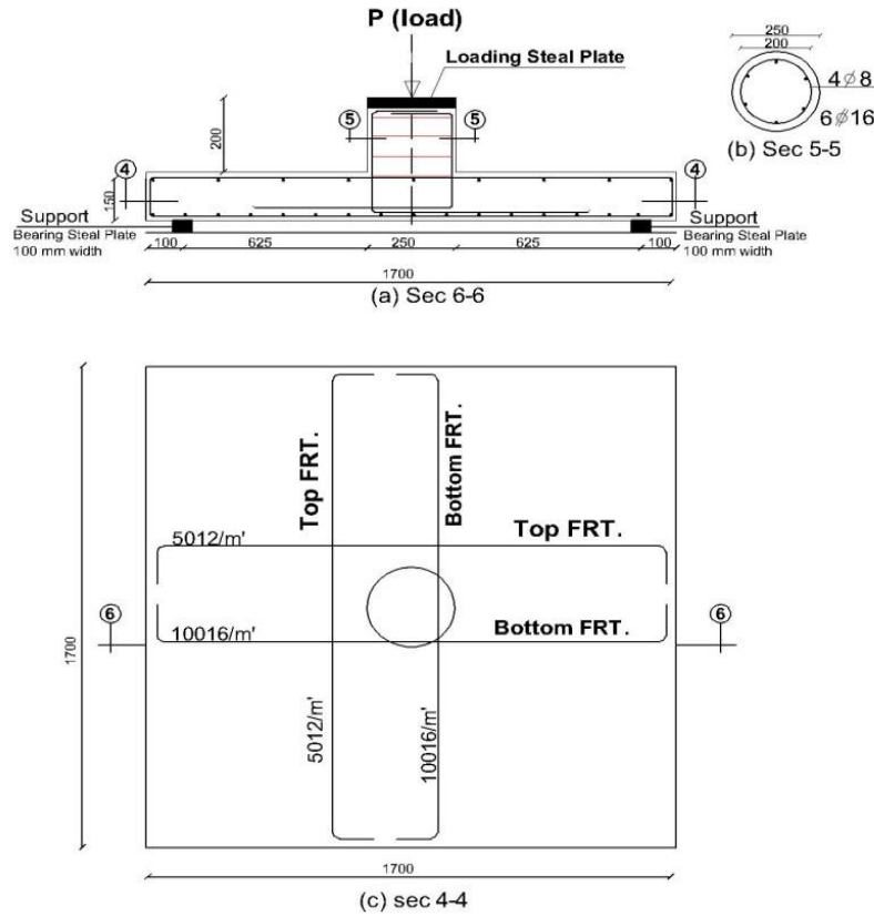
Fig. 3 Typical dimensions and reinforcement details of slab Sc [27].
