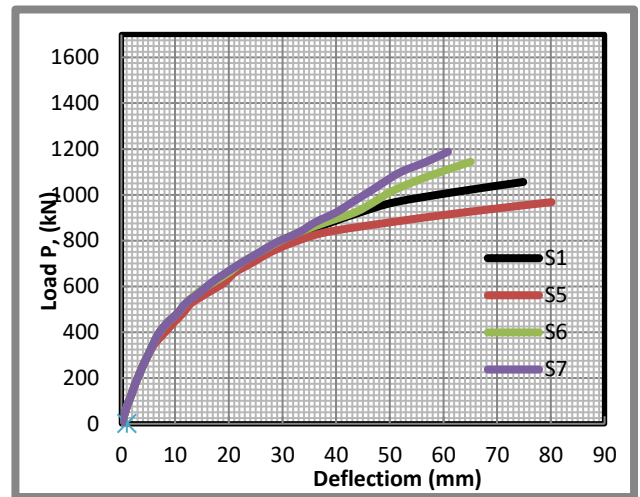
(b) Effect of reinforcement yield strength ( f_y )
