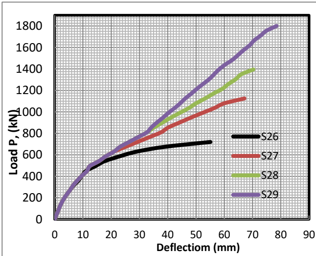
(i) Effect of drop thickness/ t_s ratio ( t_d/t_s )
